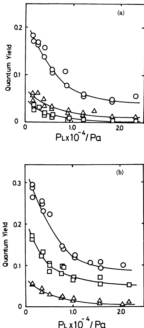
Fig. 1. Pressure dependence of quantum yields of carbon monoxide (○), ethylene (Δ), and propylene (□) in the cadmium-photosensitized reaction of (a) VL and (b) ML.
