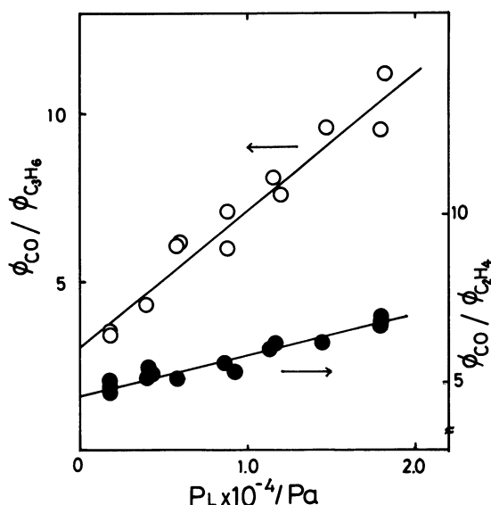
Fig. 4. Plots of \phi_{CO}/\phi_{C_3H_6} (○) for VL and \phi_{CO}/\phi_{C_2H_4} (●) for against lactone pressure.
